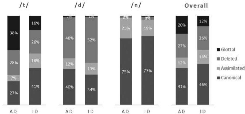
Fig. 1. Percentage of tokens classified as Canonical, Assimilated, Deleted, or Glottal as a function of Condition (ID, AD) and Segment (/t/, /d/, /n/, overall).
